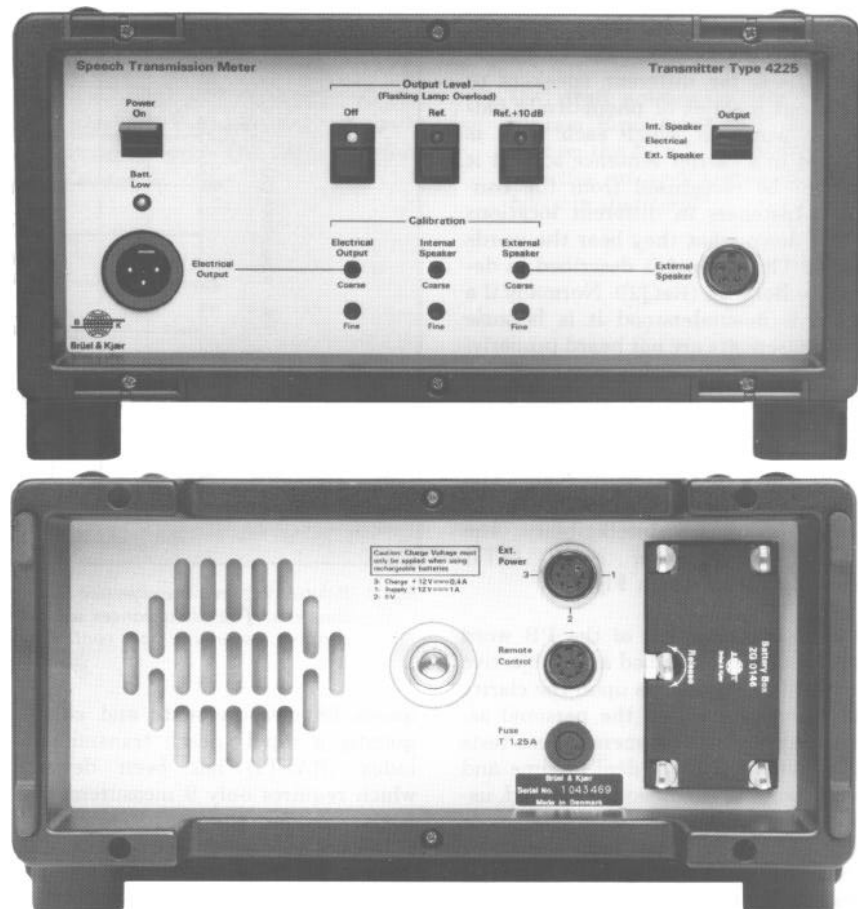
Fig. 3. Front and rear panels of the Speech Transmission Meter, Transmitter 4225. Note the loudspeaker on the left of the rear panel
