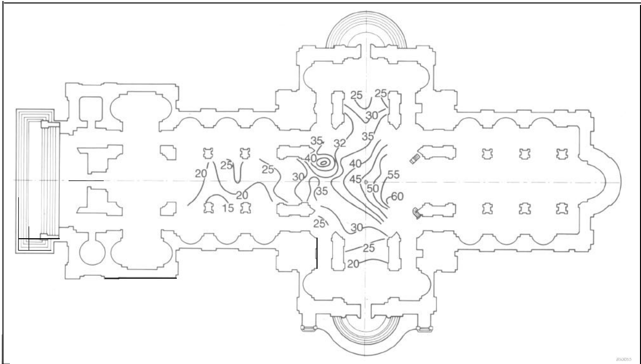
Fig. 9. The iso-RASTI contours for the source in the pulpit without reinforcement (maximum value = 45)
