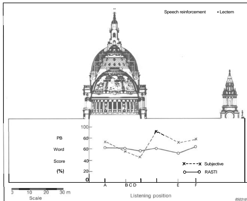
Fig 8b Comparison of results for the Transmitter placed at the lectern, with speech reinforcement
