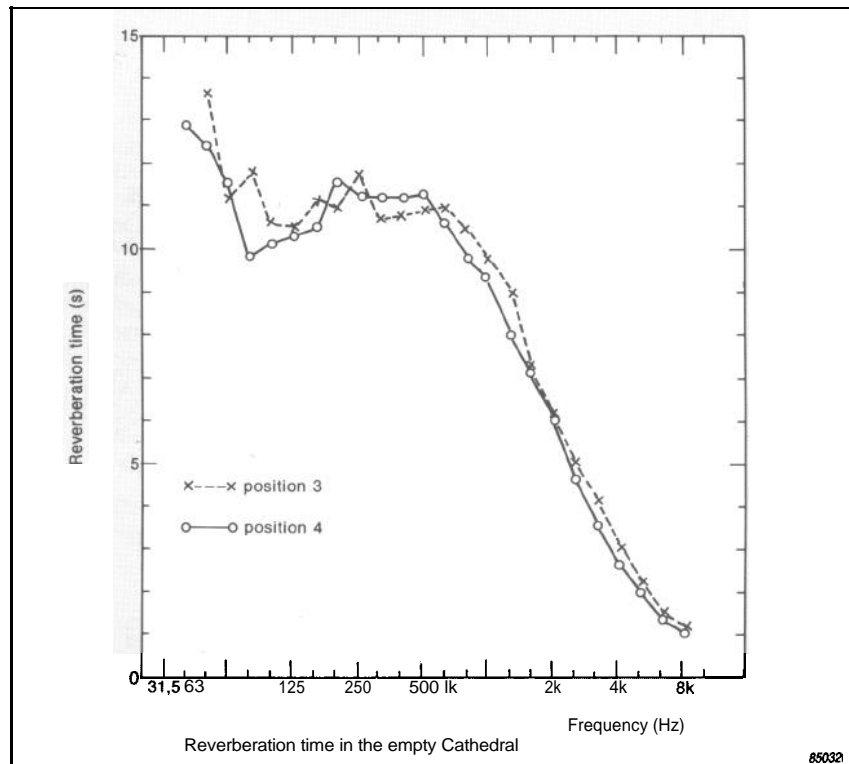
Fig 11. Reverberation time in the empty Cathedral
