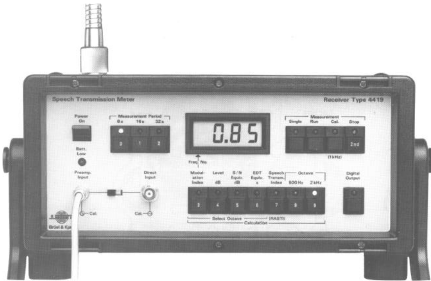
Fig. 4 Front panel of the Speech Transmission Meter, Receiver 4419
