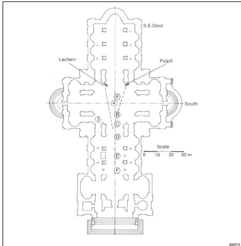
Fig. 6. Plan of the Cathedral showing the measuring positions
