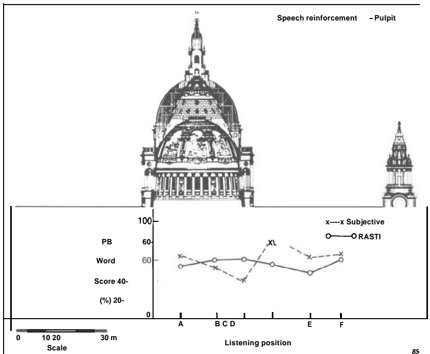
Fig 7b. Comparison of results for the Transmitter placed at the pulpit, with speech reinforcement
