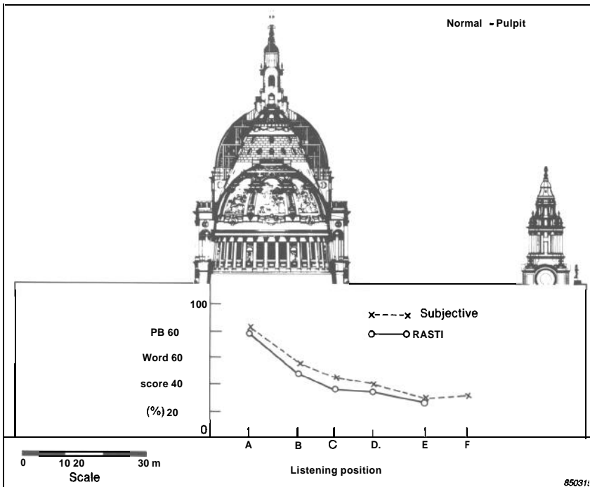
Fig. 7a. Comparison of results for the Transmitter placed at the pulpit, without speech reinforcement
