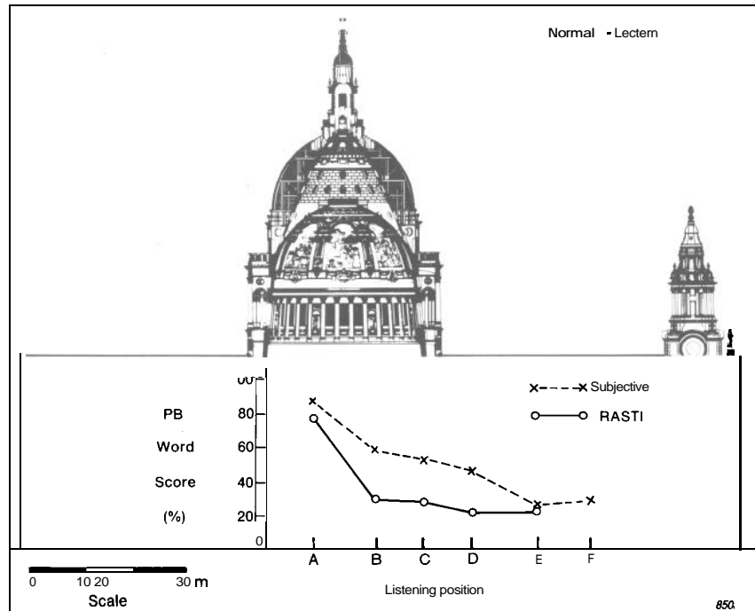
Fig 8a Comparison of results for the Transmitter placed at the lectern, without speech reinforcement
